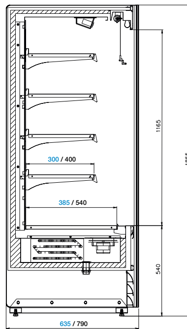
Clipper VBN / Clipper VBN slim
