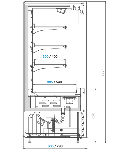
Clipper / Clipper slim
