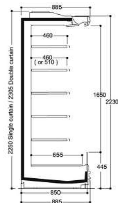
N 22 / Front 445 Glas
