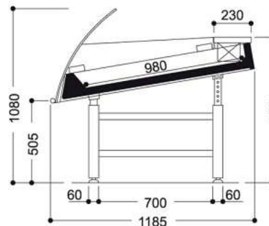
RCB With "evaporator" RCB With "serpentino" + Evaporator
